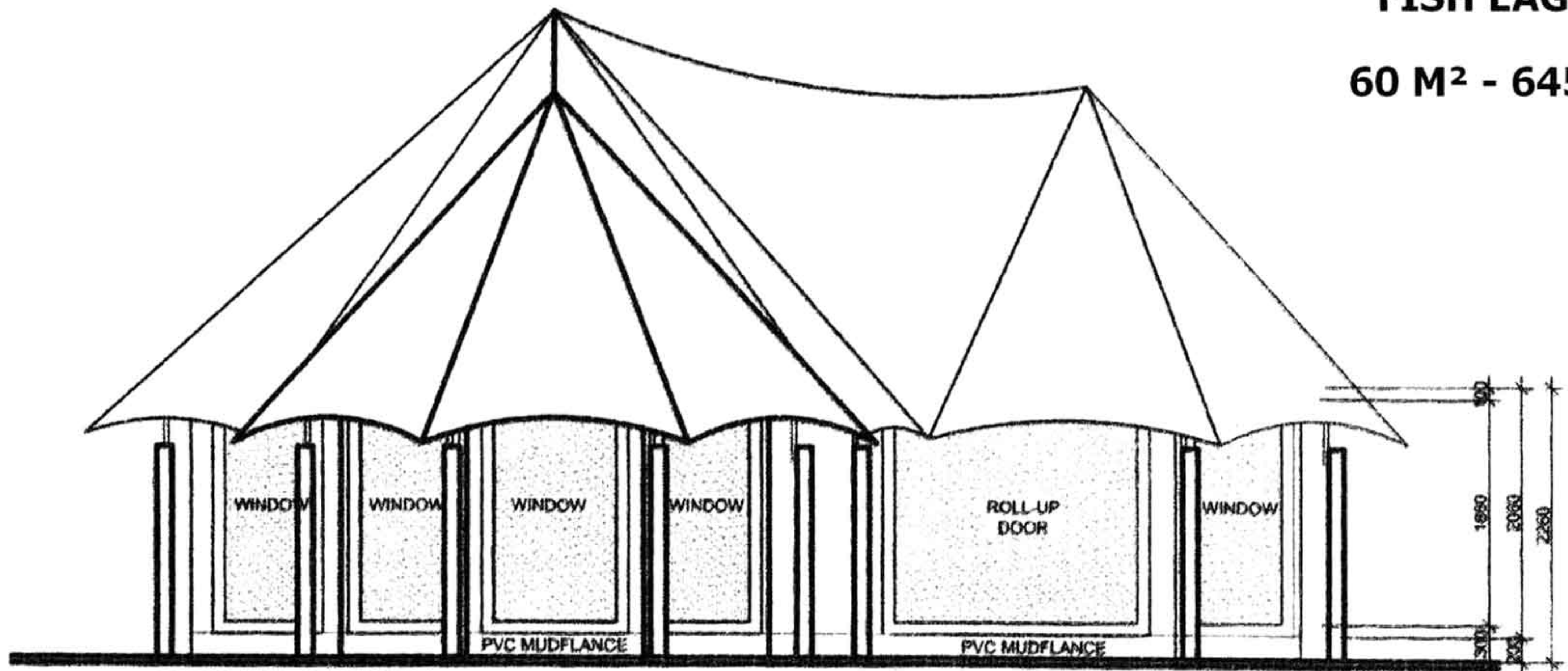
SIDE ELEVATION
