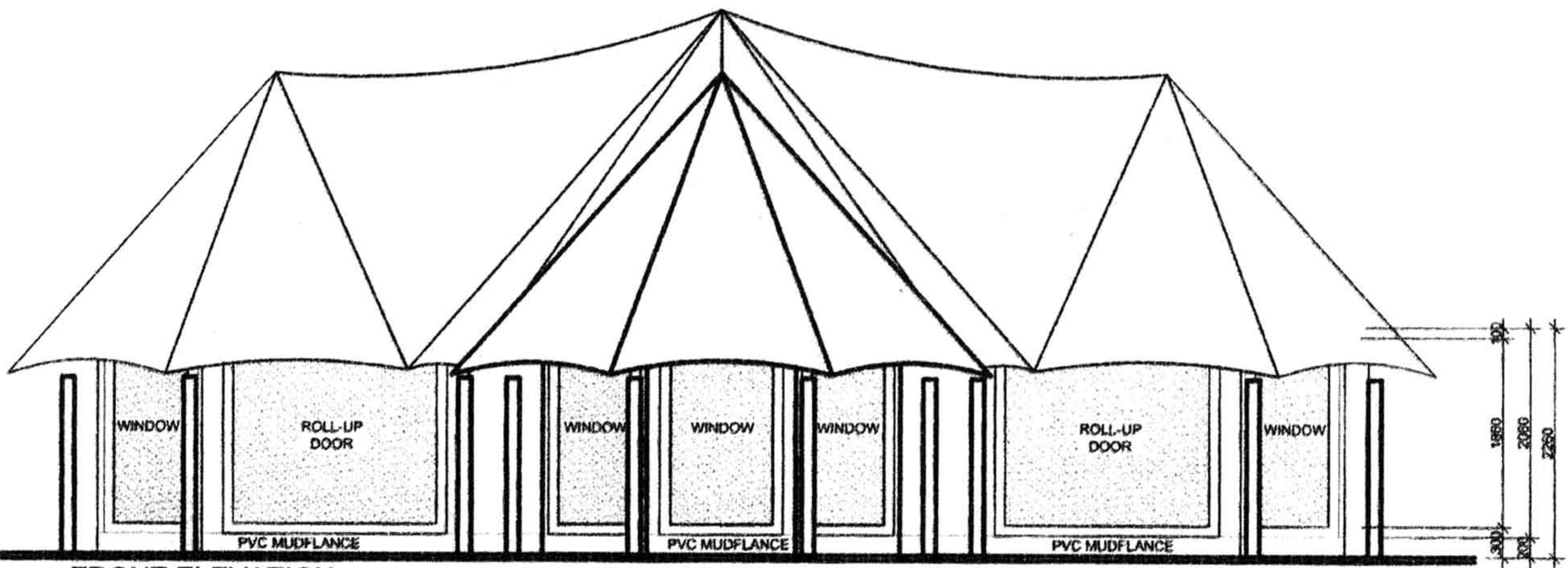
FRONT ELEVATION
